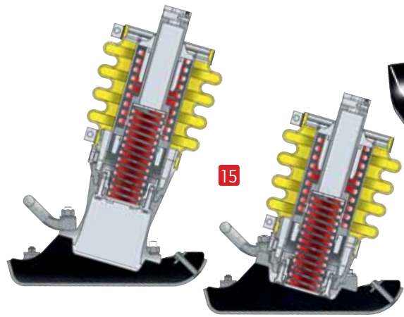
Option: reduction of machine height by approx. 10 cm by a special adapter plate
