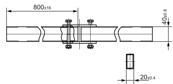
CONNECTOR BAR
