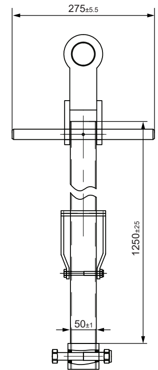
HAND LEVER
